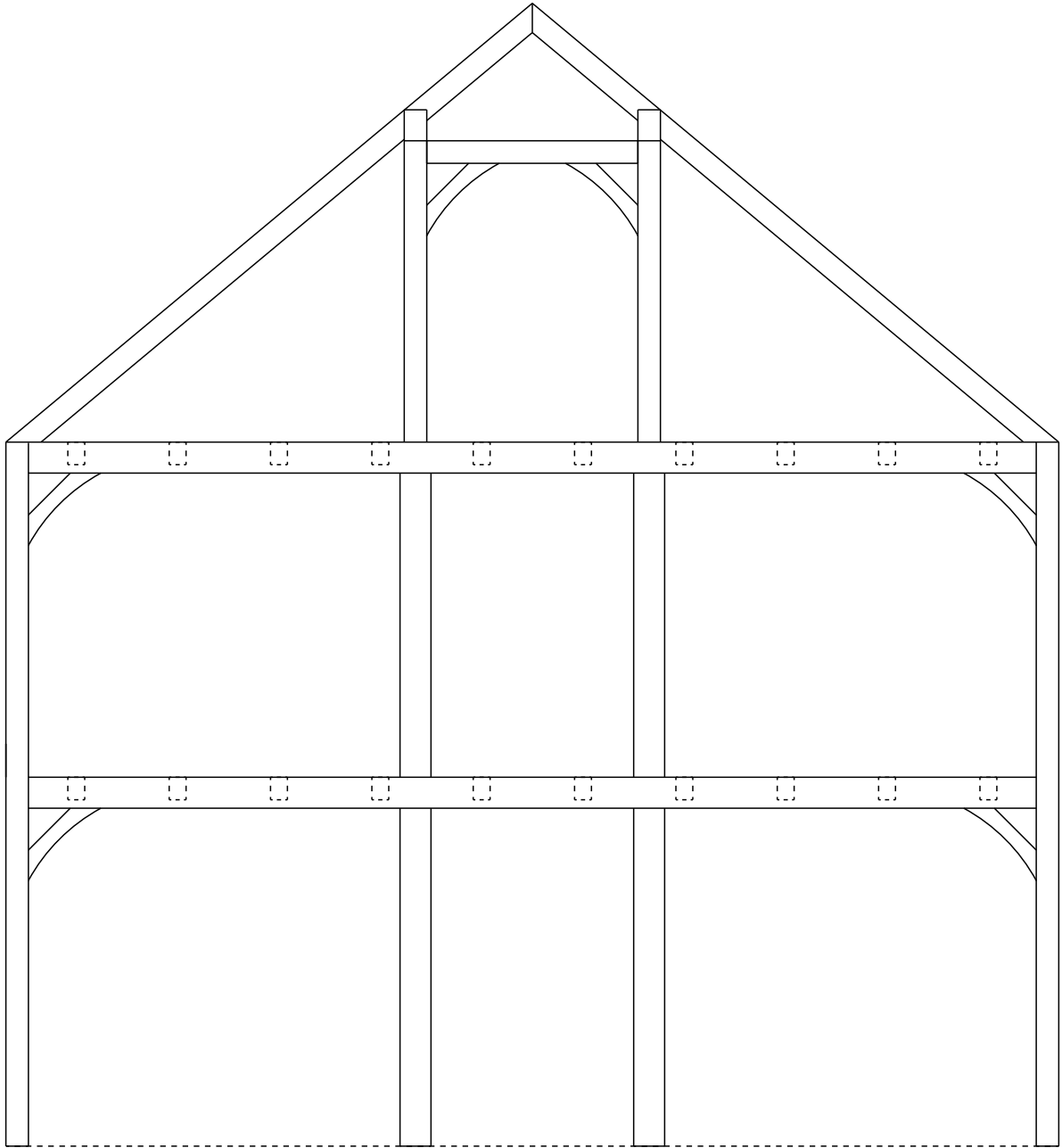
QUEEN POST DESIGN
